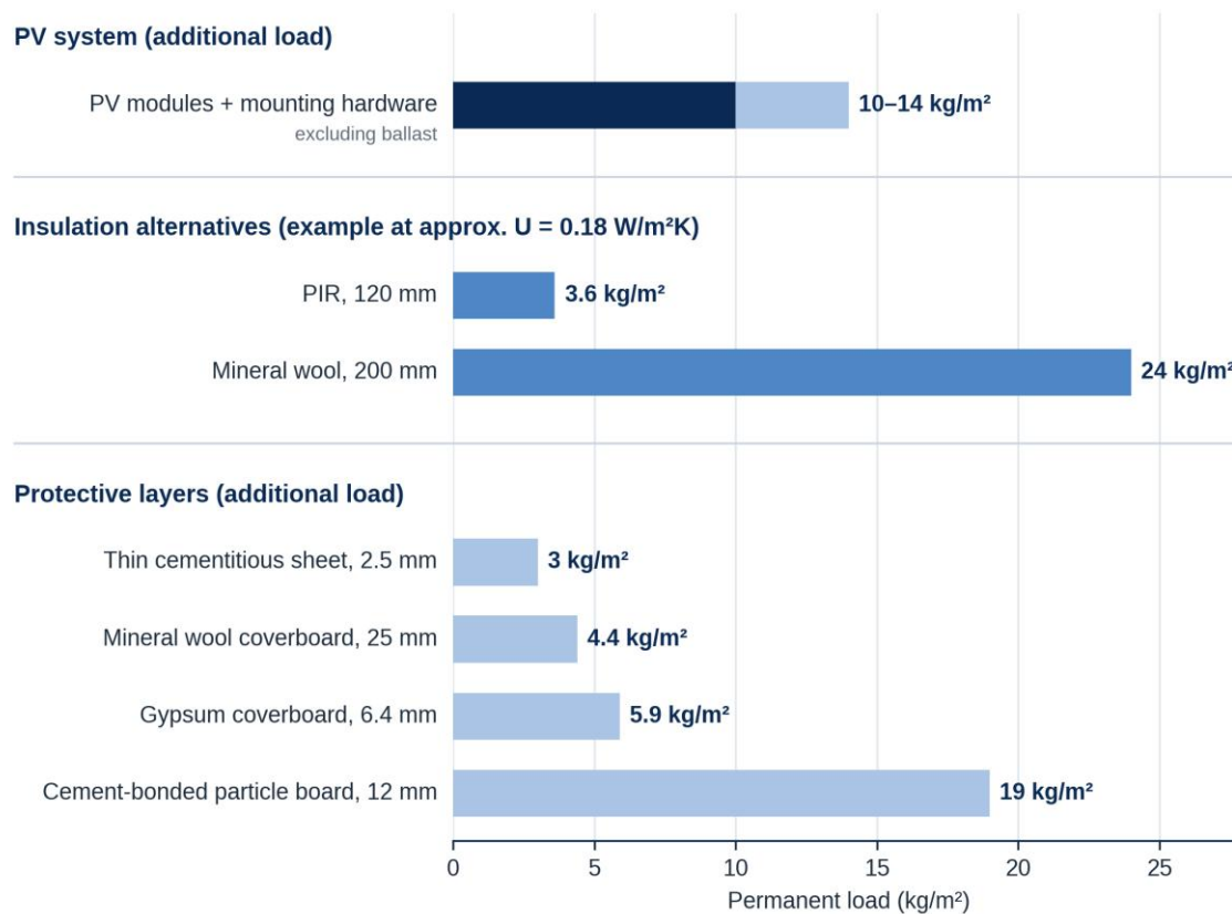
Figure 3. Illustrative permanent roof loads. Insulation alternatives replace one another while protective layers represent additional load.
