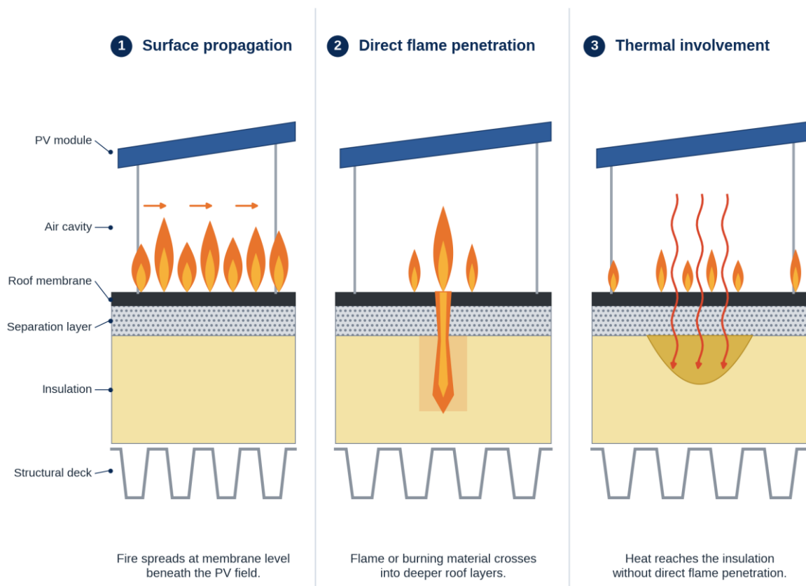
Figure 1. Surface propagation, direct flame penetration and thermal involvement are different outcomes in a rooftop PV fire.
